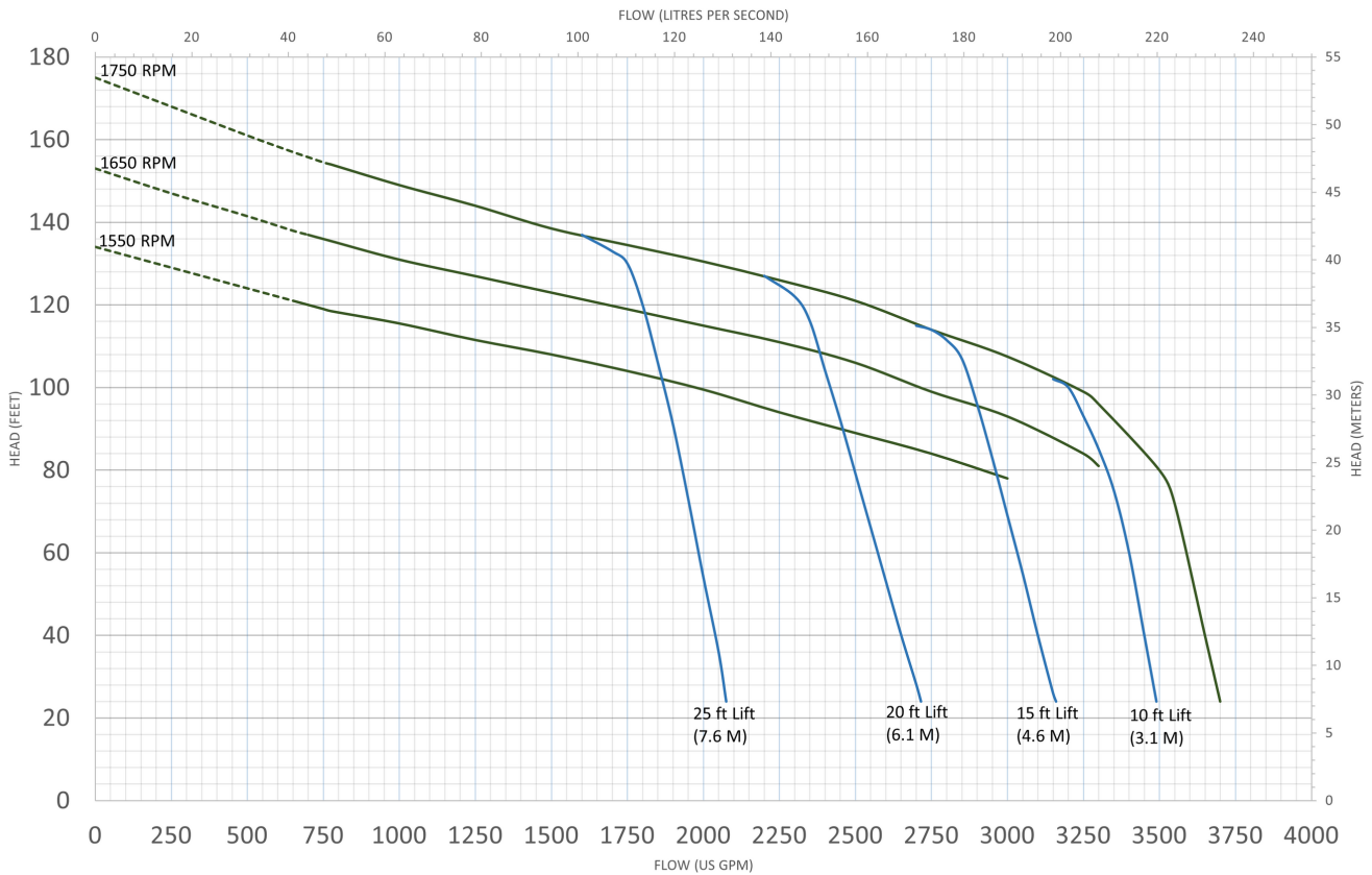
10" x 10" Self Prime Pump w/ 173 HP Engine Performance Curve
